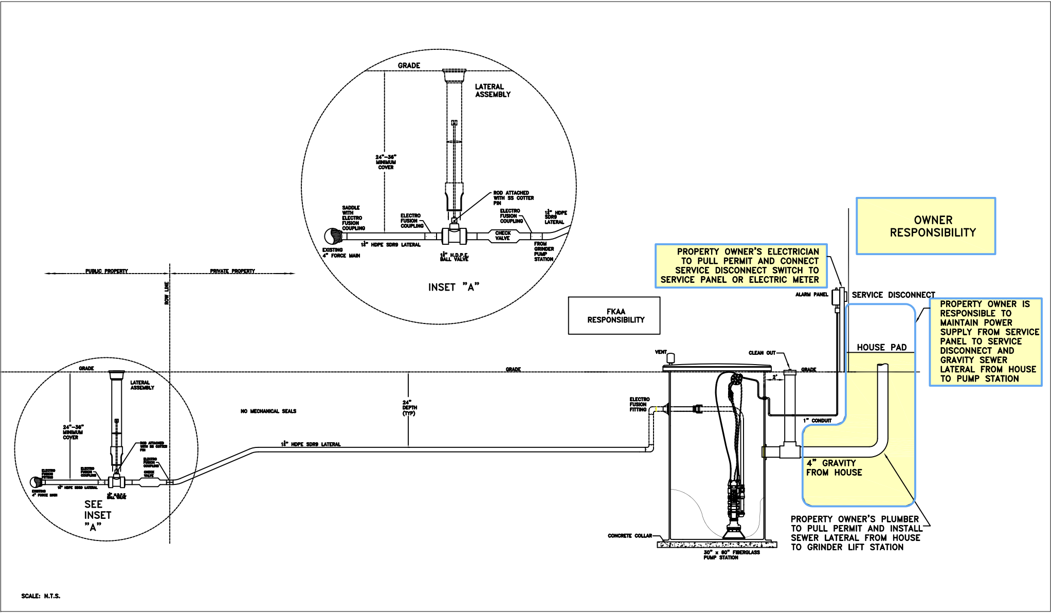
FLORIDA KEYS AQUEDUCT AUTHORITY CENTRAL CUDJOE REGIONAL W.W. COLLECTION SYSTEM CUDJOE KEY LPS GRINDER PACKAGE TYPICAL SITE INSTALLATION
